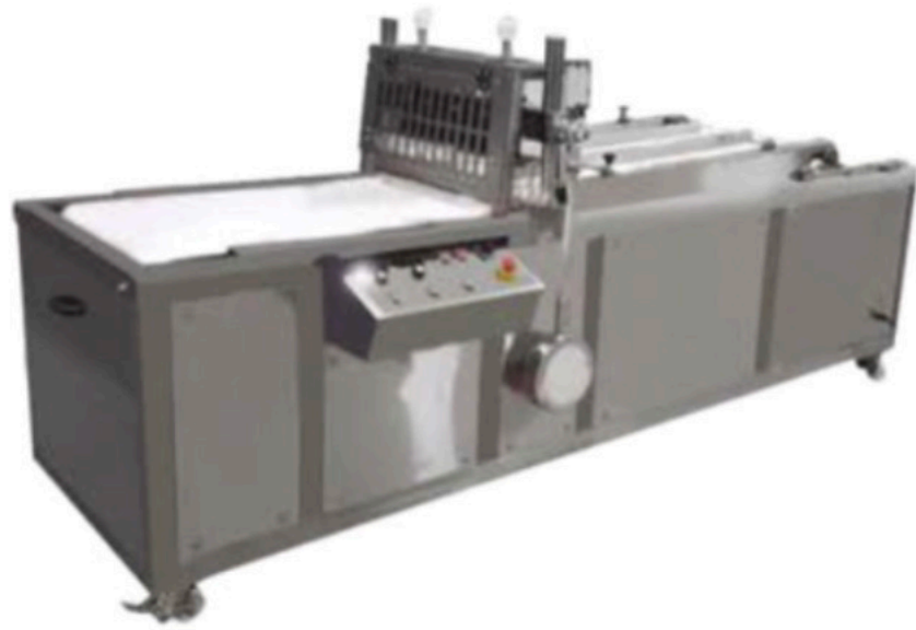
OTOMATİK BANTLI LOKUM KESME MAKİNASI INV LK 01 AUTOMATIC CUTTING MACHINE WITH BAND SYSTEM
